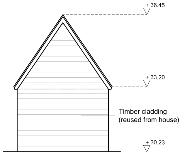
3. SOUTH ELEVATION 1:100 @ A3
