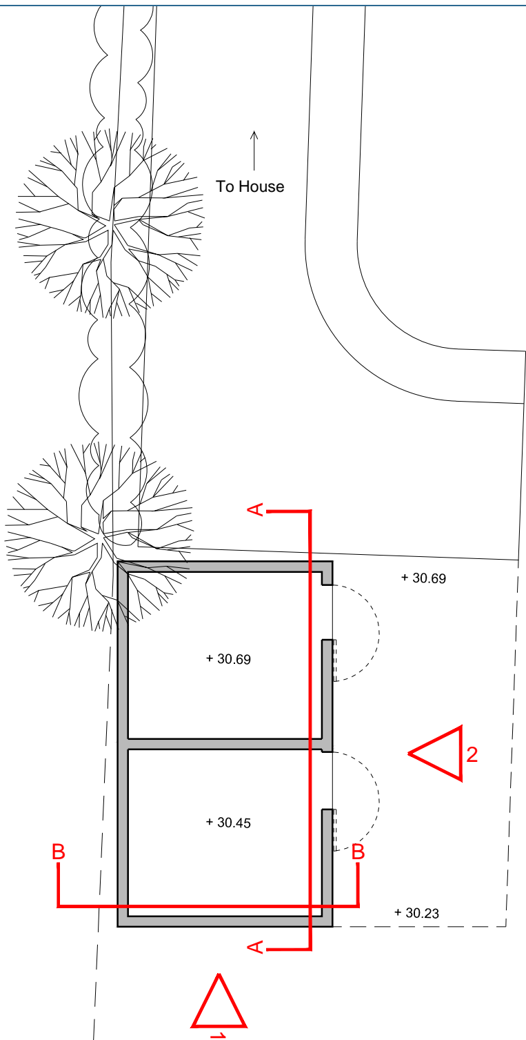
1. GROUND FLOOR PLAN 1:100 @ A3
