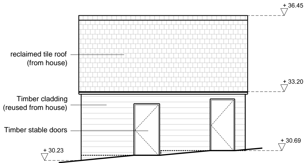
2. EAST ELEVATION 1:100 @ A3
